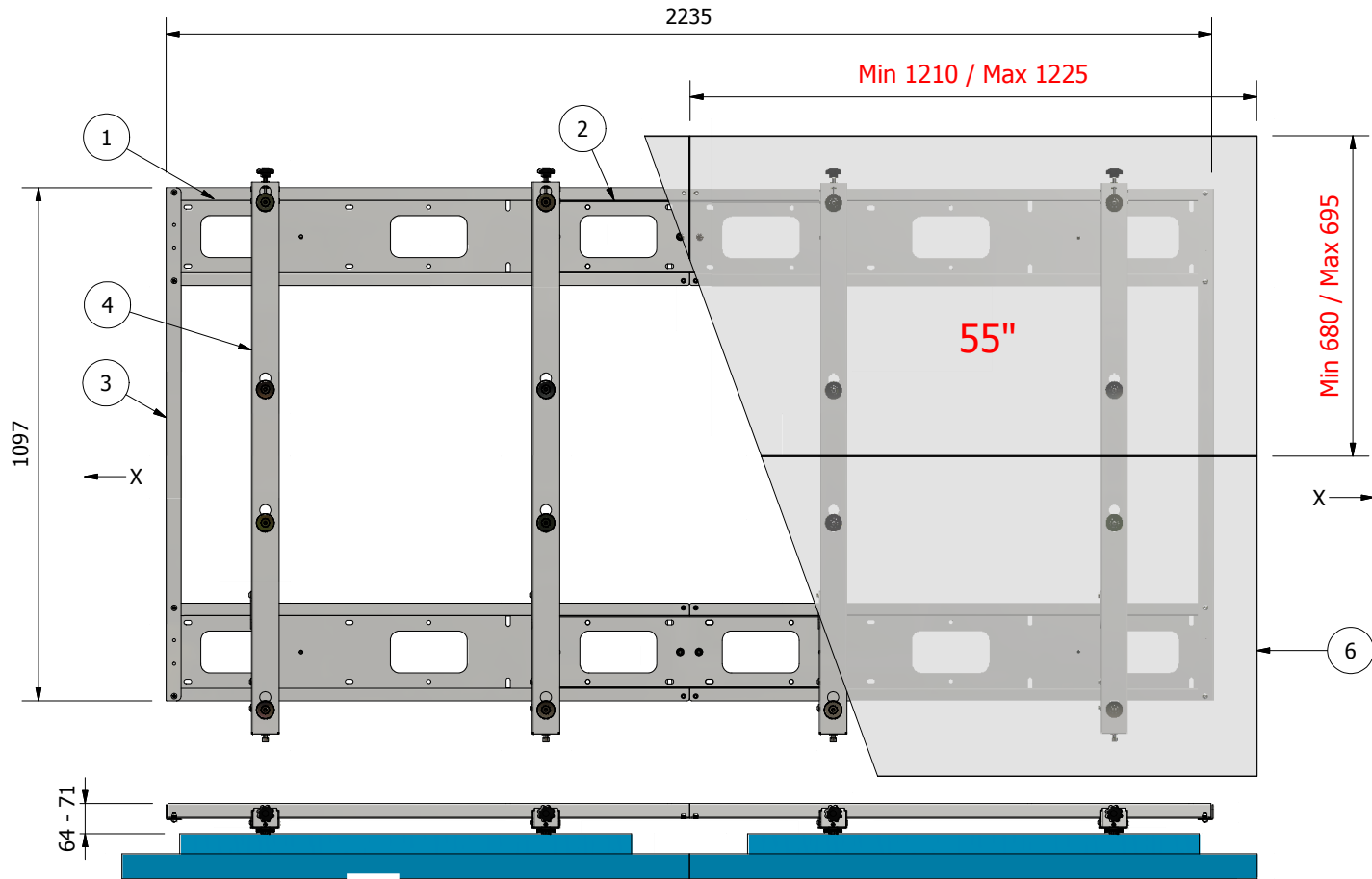
Quick mounting
